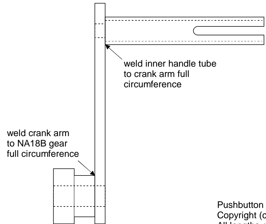
crank assembly
